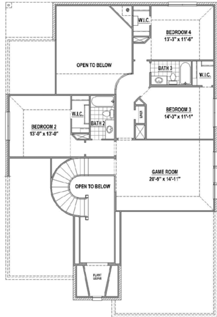
Second Floor
